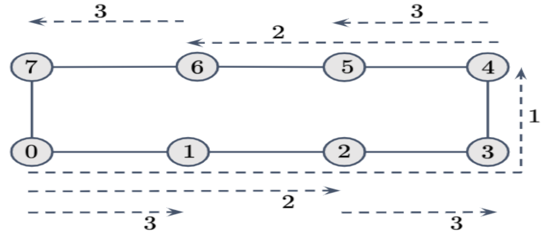
One-to-all broadcast
