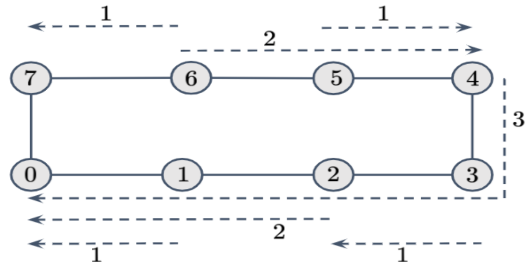
All-to-one reduction
